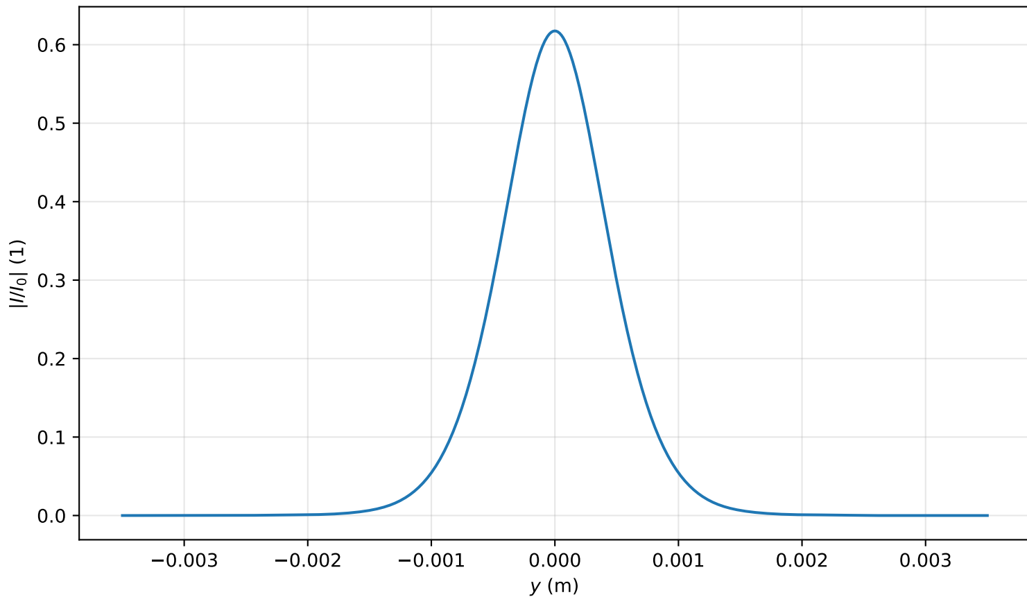
Intensity profile I(x=0, y, z=3.264)/I_0 , \text{Pin}=0.6P_{\text{cr}} , artificial time
